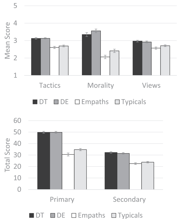
Fig. 4. Mean scores from study 3 for Machiavellianism (top panel) and psychopathy (bottom panel) as a function of latent class. Error bars denote standard error.
