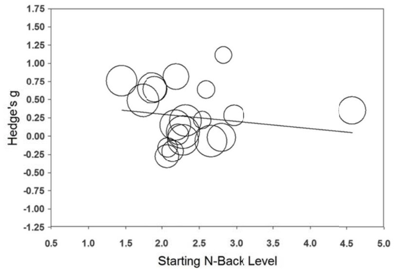
Fig. S3b. Regression Plot of Starting n-back level (Original)
