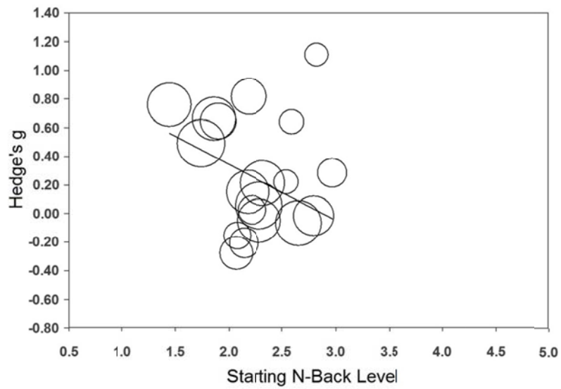
Fig. S3a: Regression Plot of Starting n-back level (Outliers Trimmed)
