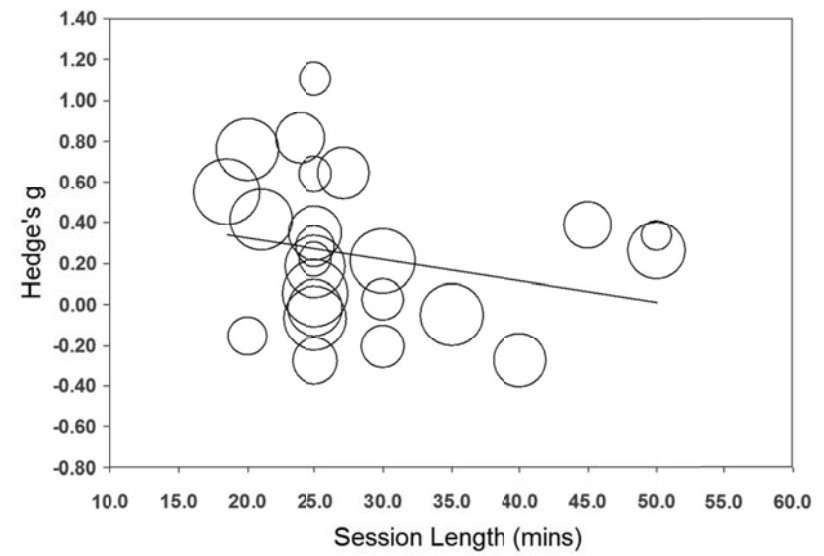
Fig. S2b. Regression Plot of Session Length (Original)
