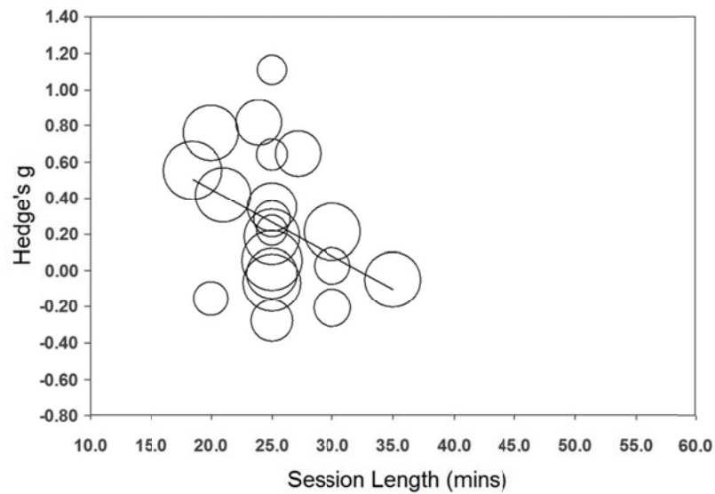
Fig. S2a. Regression Plot of Session Length (Outliers Trimmed)
