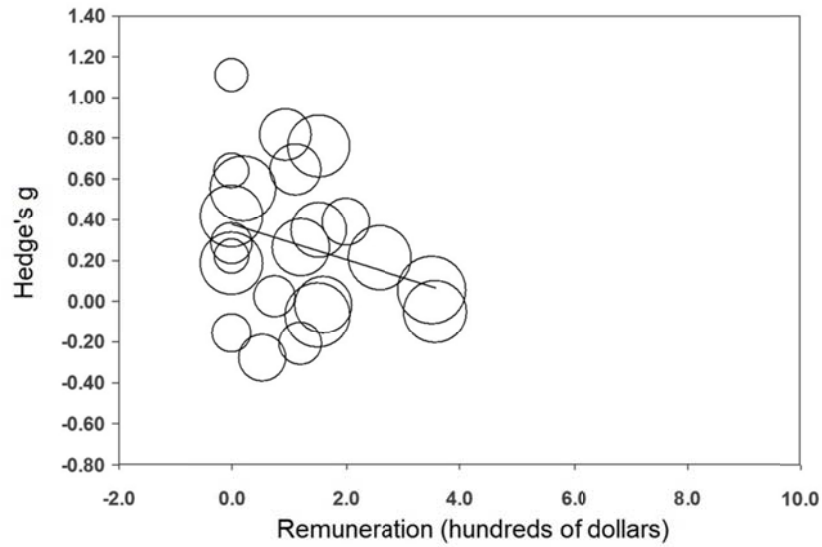
Fig. S1a. Regression Plot of Remuneration (Outliers Trimmed)
