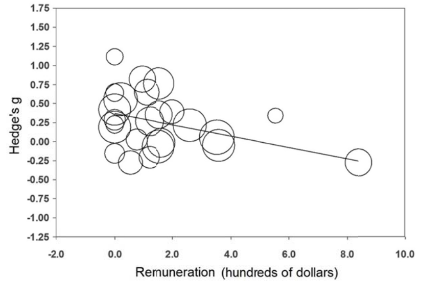
Fig. S1b. Regression Plot of Remuneration (Original)
